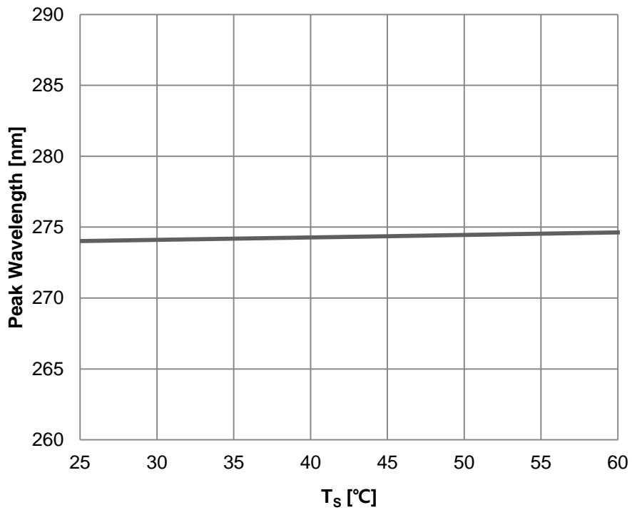
Fig 6. Surface Temperature vs. Peak Wavelength, I_F=100\text{mA}
