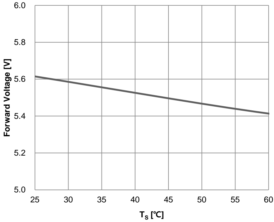
Fig 7. Surface Temperature vs. Forward Voltage, I_F=100\text{mA}
