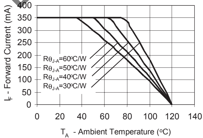
Figure 5c. Maximum Forward Current vs. Ambient Temperature. Derating based on T_{J\text{MAX}} = 120^{\circ}\text{C} for Warm White.
