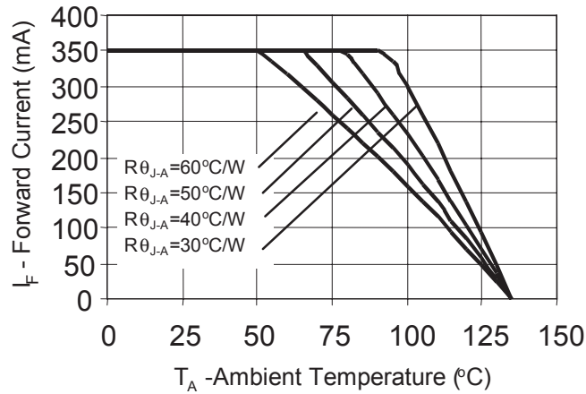
Figure 5a. Maximum Forward Current vs. Ambient Temperature. Derating based on T_{J\text{MAX}} = 135^{\circ}\text{C} for White, Green, Cyan, Blue, and Royal Blue.
